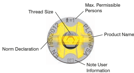
Image 2: Identification on Sleeve and Screw. Component description and location of identification details on product.
