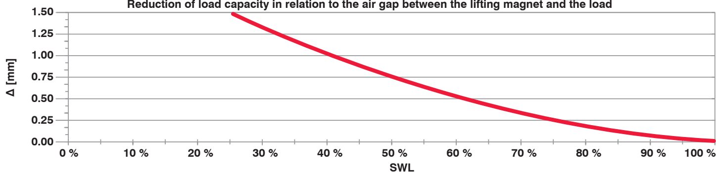
Reduction of load capacity in relation to the air gap between the lifting magnet and the load
